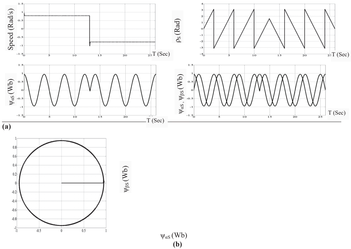
Fig. 7 Simulation results of the proposed DTC-AAS during speed reversal peration at 0.25 Hz ( \pm 7,5 rpm). (a) speed, Stator flux angle and \alpha -axis flux; (b) \alpha\beta -axis and stator flux trajectory.
