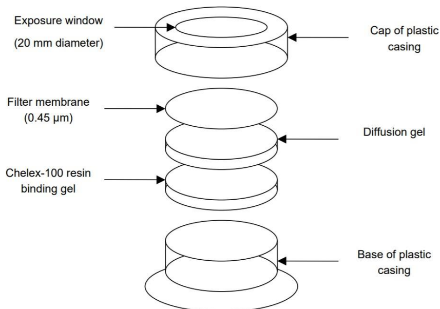
Figure 2. DGT assembly
